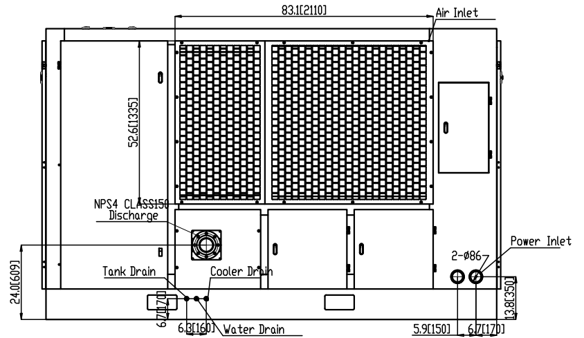
View A
