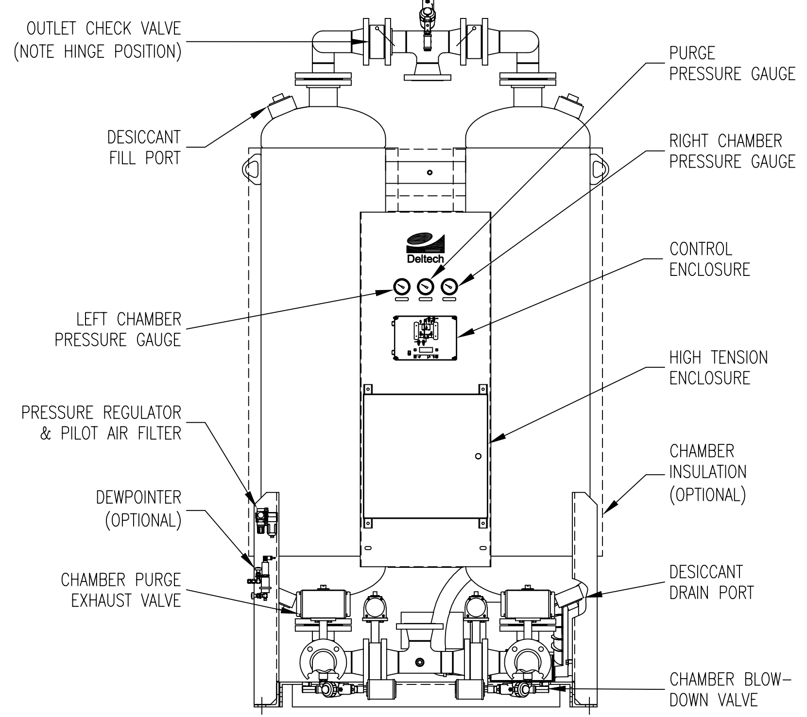
FRONT VIEW
