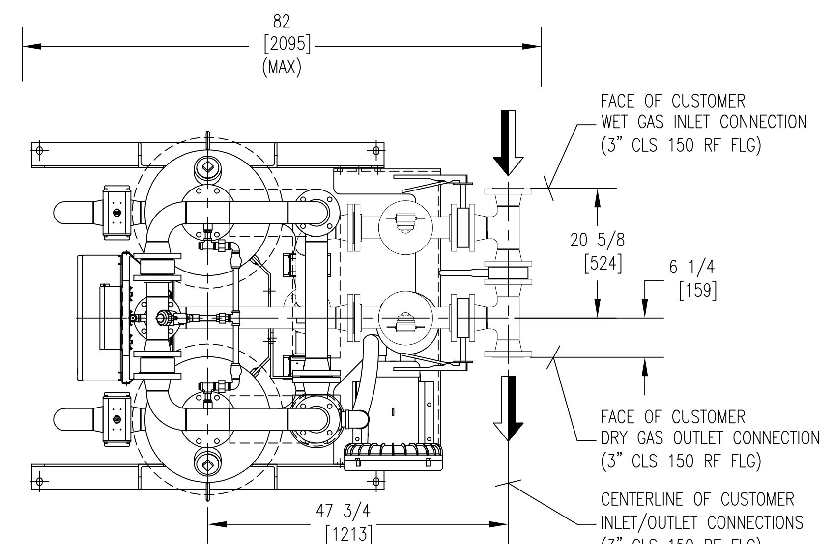
TOP VIEW (F02 PKG OPTIONAL)
