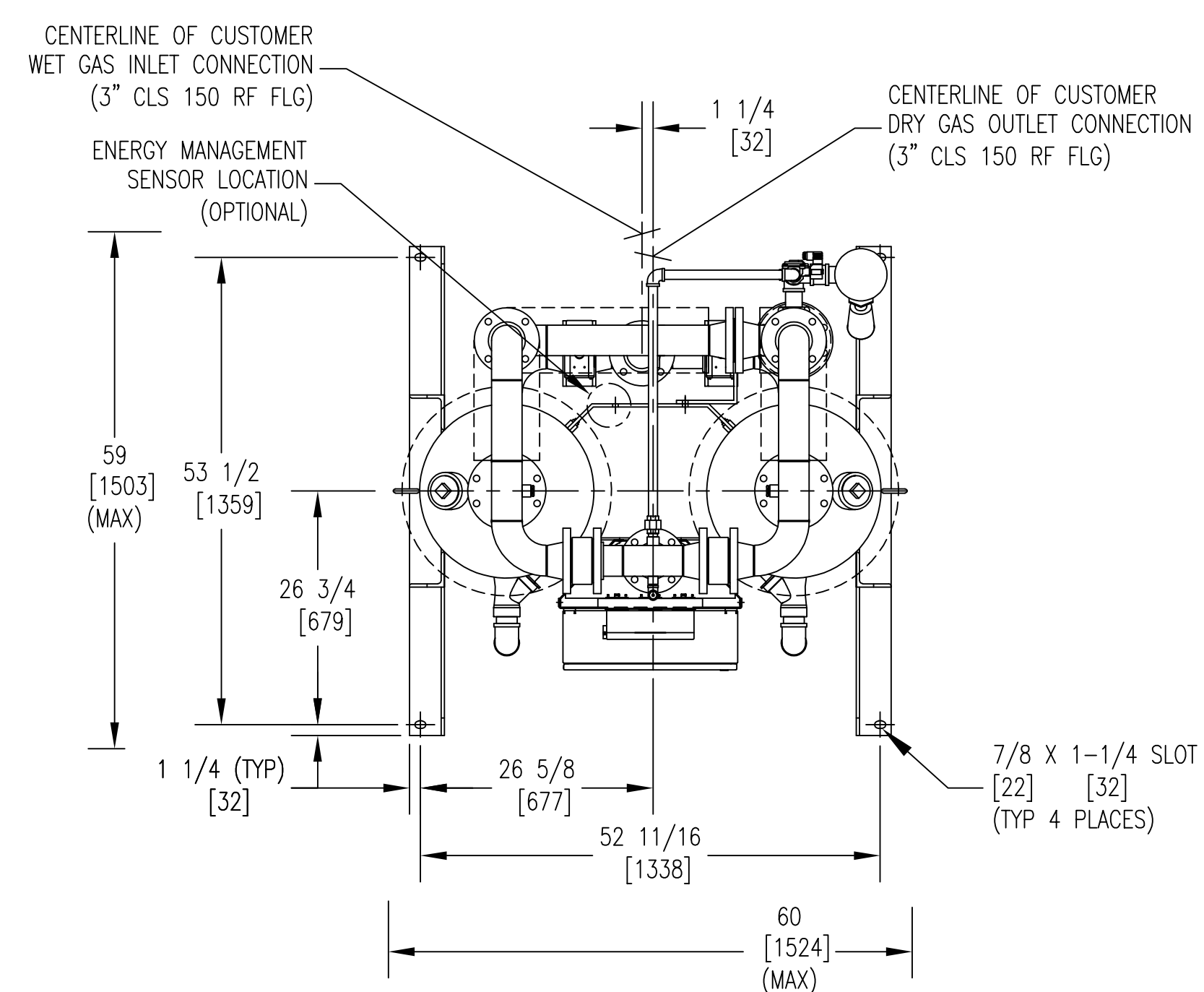
TOP VIEW
