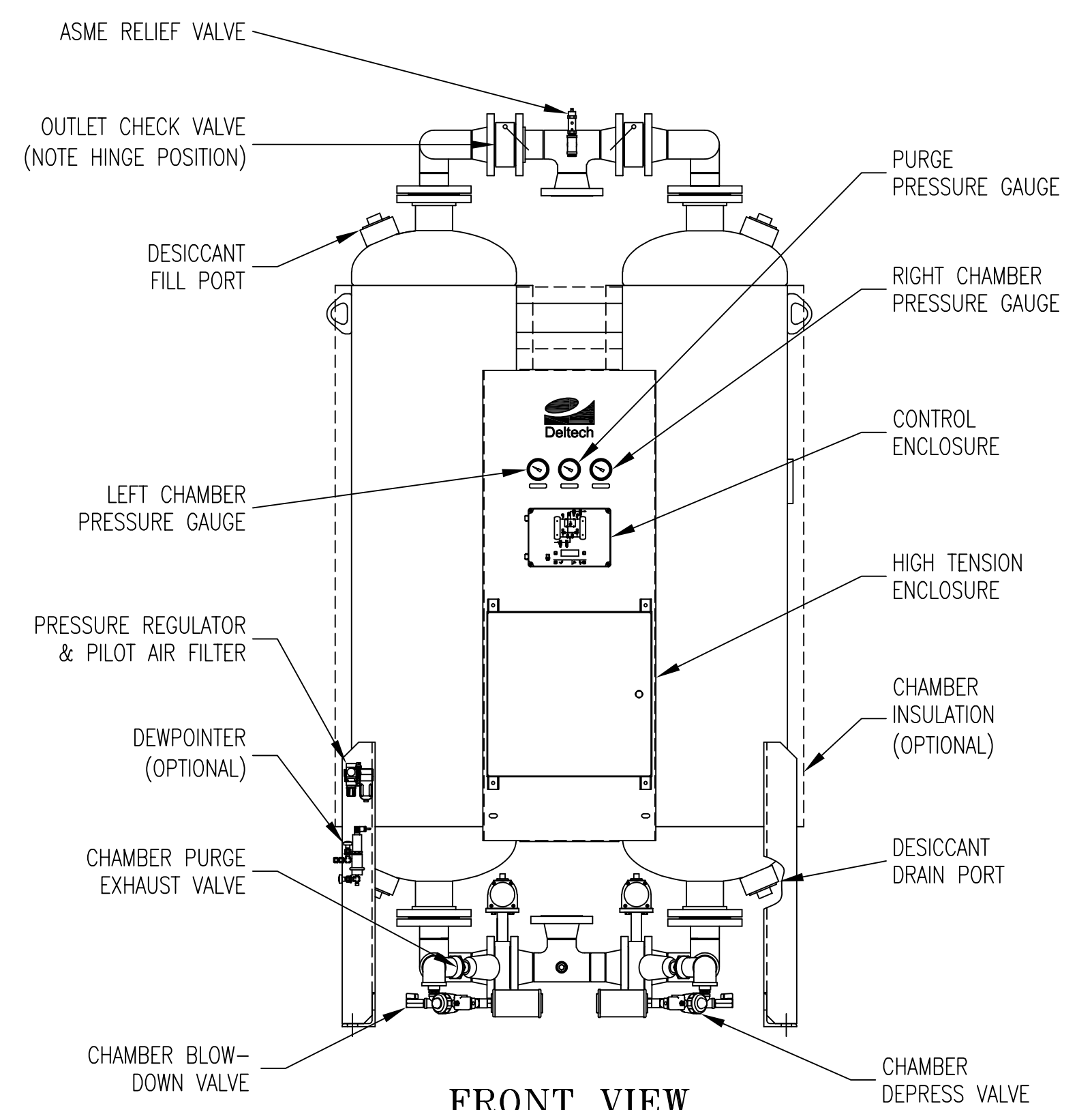
FRONT VIEW
