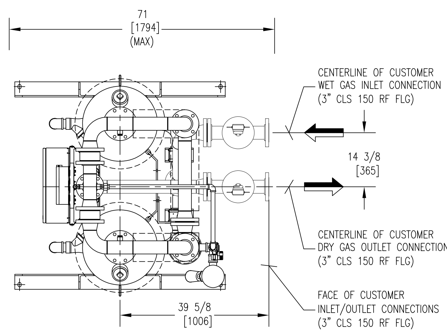
TOP VIEW (F01 PKG OPTIONAL)
