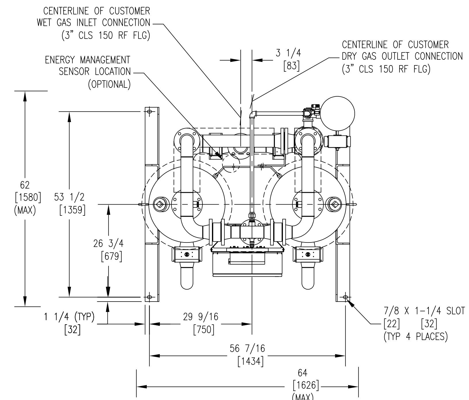
TOP VIEW
