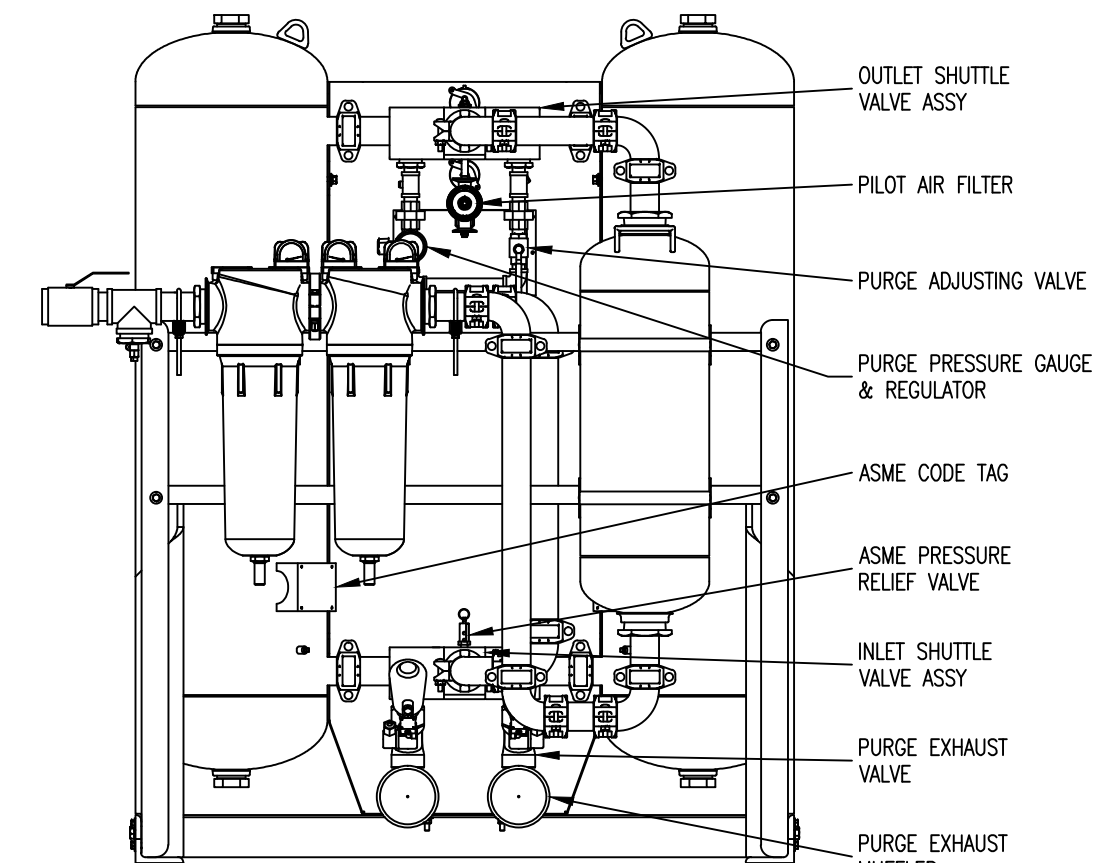
REAR VIEW
