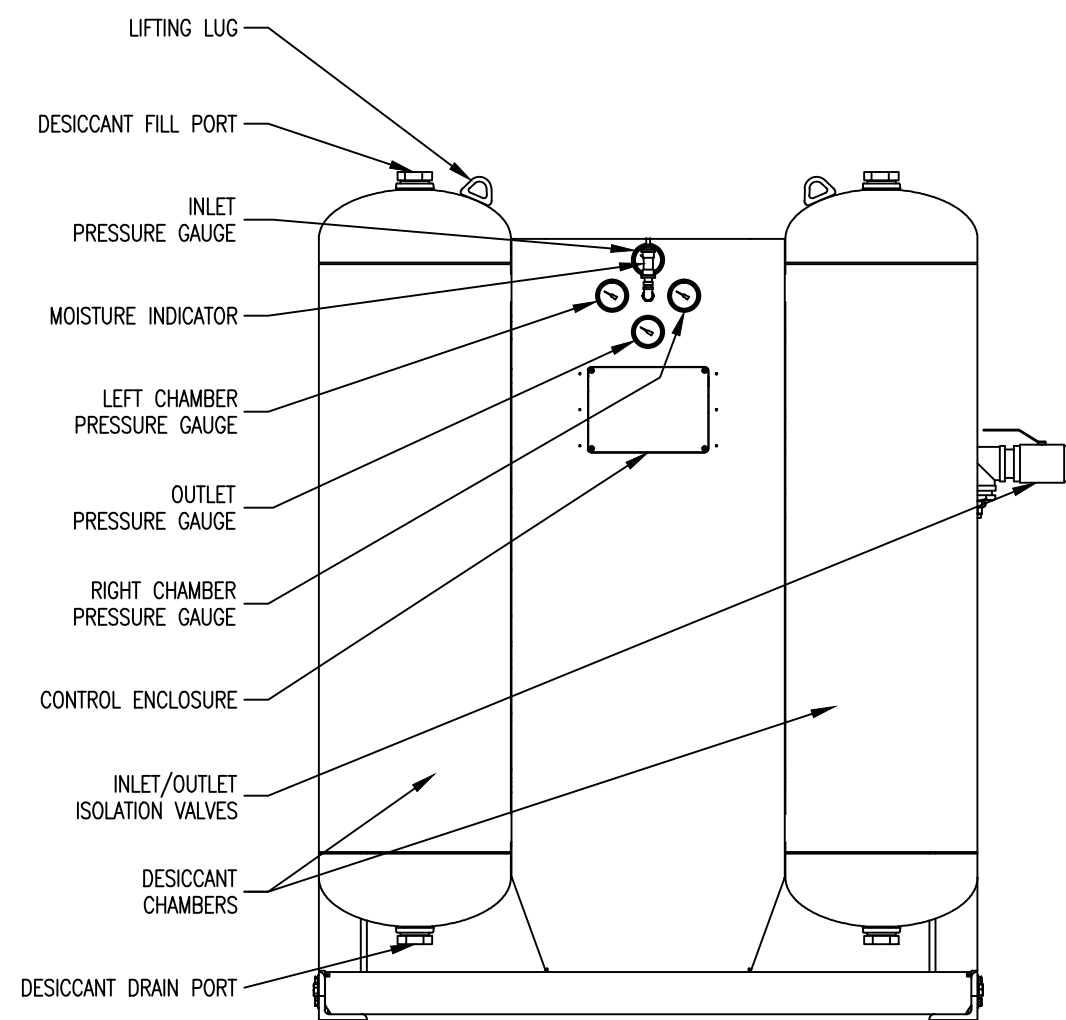
FRONT VIEW
