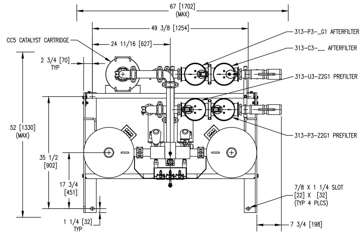
TOP VIEW
