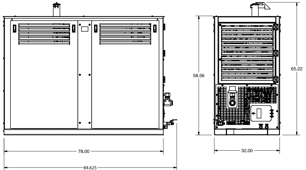
BOSS FT4 DUS Dimensions
